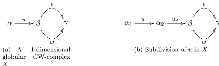
Figure 12: Example of temporal deformation
