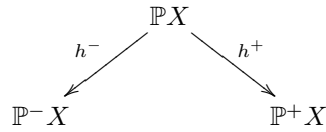
Figure 15: The fundamental diagram for a globular CW-complex X
