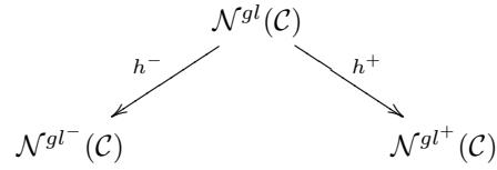
Figure 14: The fundamental diagram
