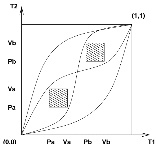
Figure 2: The progress graph corresponding to Pa.Va.Pb.Vb \mid Pa.Va.Pb.Vb
