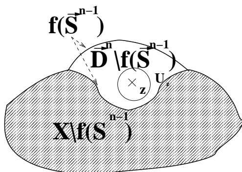
Figure 7: First case for the definition of (U_z, \prec_{U_z}) .
