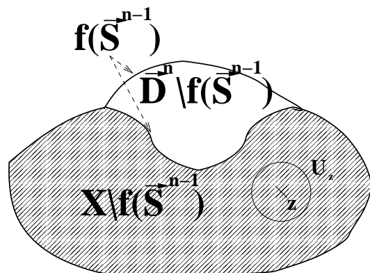
Figure 8: Second case for the definition of (U_z, \prec_{U_z}) .
