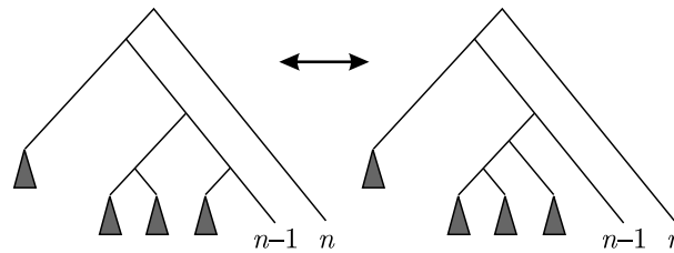
Figure 4. Another elementary manipulation.
