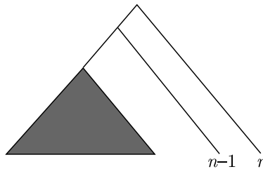
Figure 5. The tree \mathbf{T}_{r_2} .
