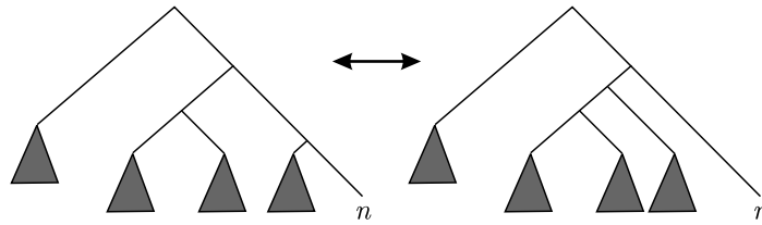
Figure 3. An elementary manipulation. The shaded triangles represent subtrees whose form is not relevant.
