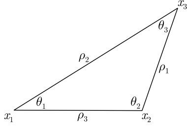
Figure 6. The triangle spanned by x_1, x_2, x_3 .
