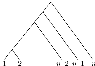
Figure 2. The reference tree \mathbf{S} .
