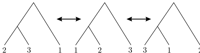
Figure 1. A graphical representation of the associativity condition. The double arrows indicate that the domains \mathcal{D}[\mathbf{T}_i] represented by the respective trees have a common intersection, and that on this intersection, the OPE's represented by the respective trees coincide. Note that the double arrows are not a transitive relation: The domains associated with left- and rightmost tree have empty intersection.
